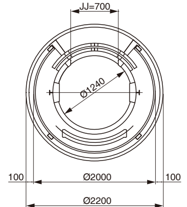
SHAFT PLAN
